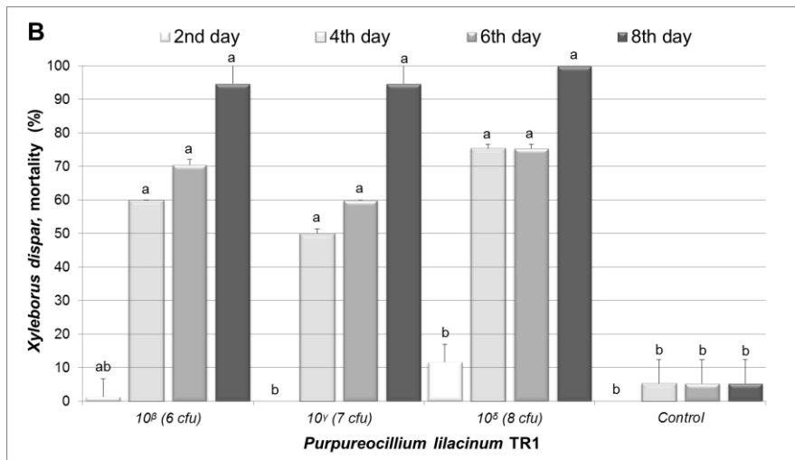
Figure 1. Mean adult mortality (%±SEM) of Xylosandrus germanus (A) and Xyleborus dispar (B) exposed for 2 nd , 4 th , 6 th and 8 th days on favored bait treated with Purpureocillium lilacinum TR1 (isolated from Turkey) (10 6 , 10 7 and 10 8 cfu ml -1 concentration) (means followed by the same letters are not significantly different at P=0.05).
